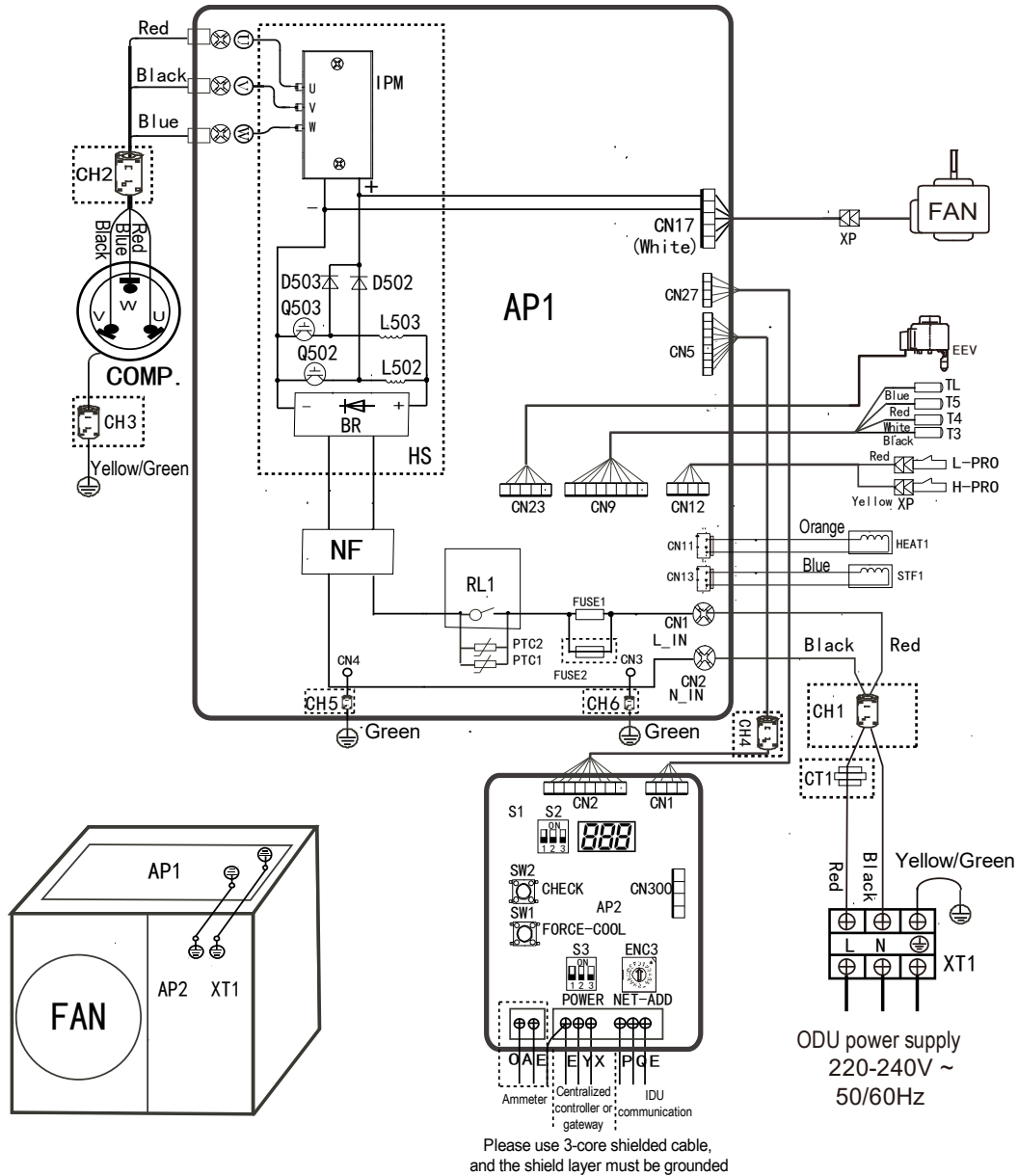
Figure 2-5.2: 100/120 model wiring diagram
