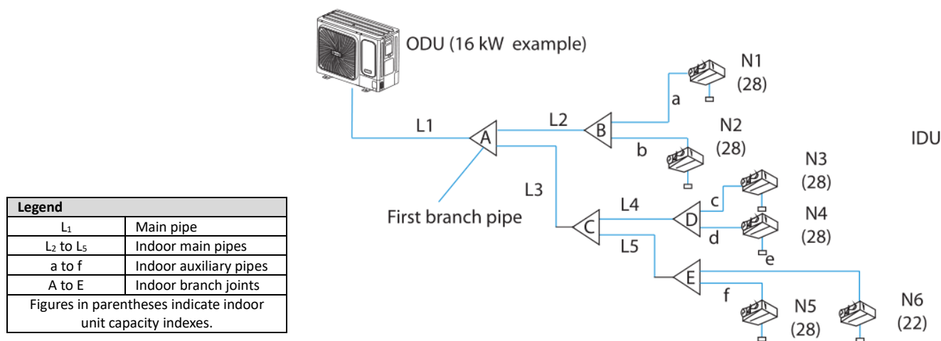
Figure 3-3.4: Refrigerant piping selection example
