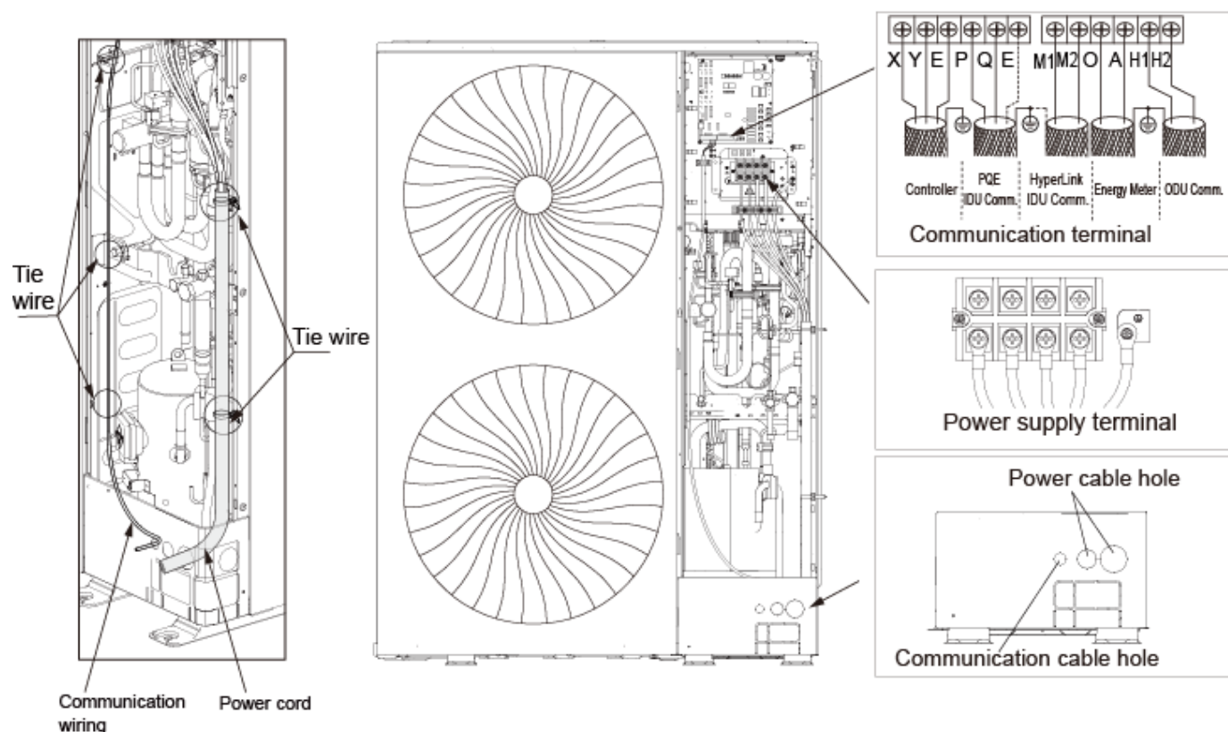
Figure 3-9.1: Wiring layout
