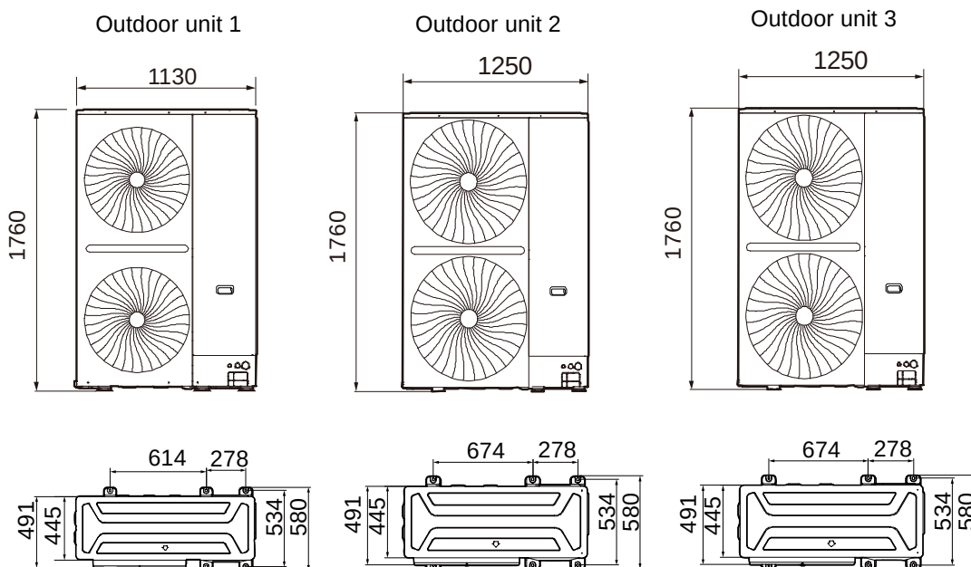
Figure 2-2.8: 50/56HP dimensions (unit: mm)
