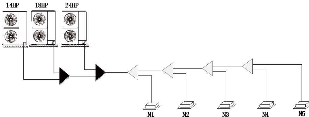
Figure 3-2.1: Positioning of master and slave units
