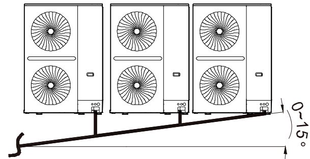
Figure 3-5.15: Piping connections inclination angle
