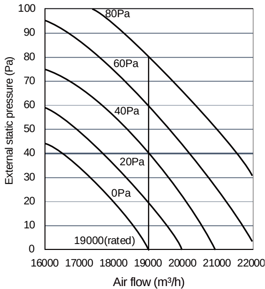
Figure 3-3.10: 24HP units fan performance
