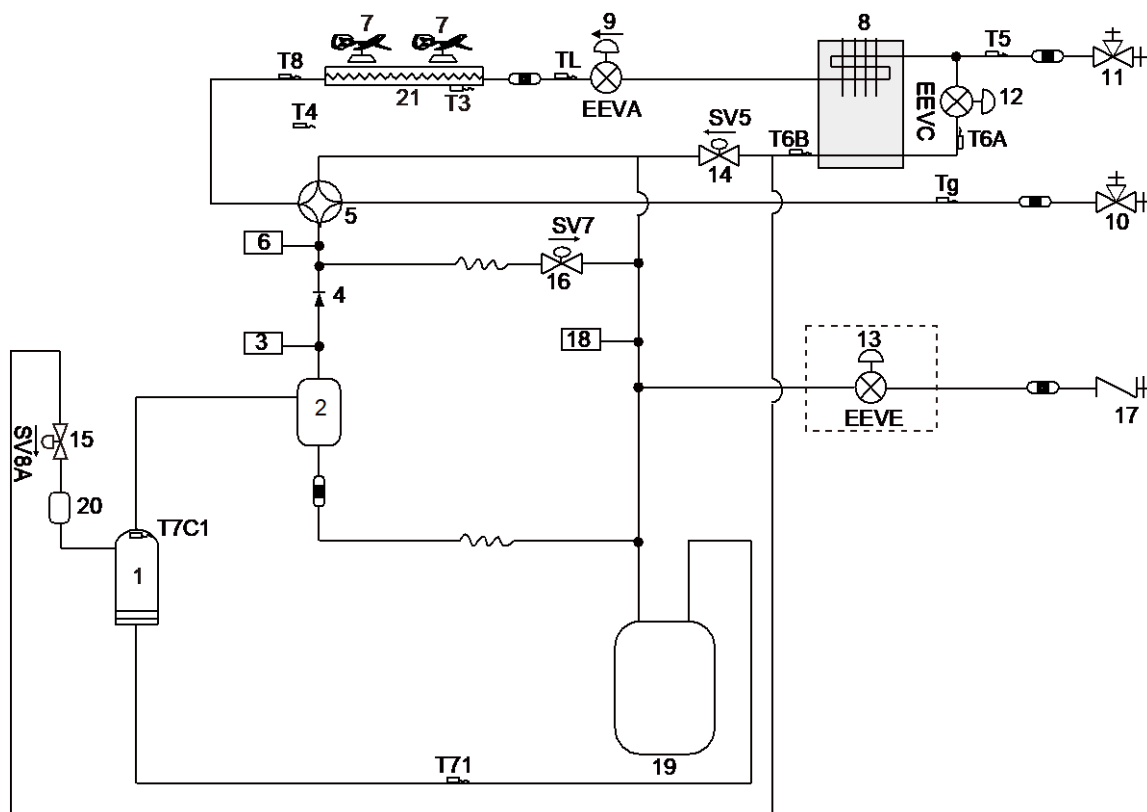
Figure 2-4.2: 16-24HP piping diagram
