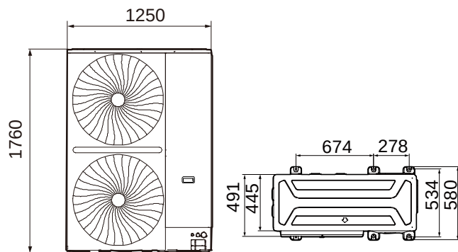
Figure 2-2.2: 16/18/20/22/24HP dimensions (unit: mm)
