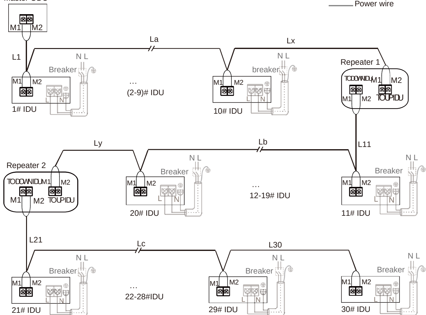
L1+La+Lx \leq 200m , L11+Lb+Ly \leq 200m , L21+Lc+L30 \leq 200mm . Communication wiring 2 \times 1.5mm^2
