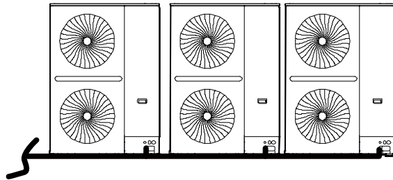
Figure 3-5.13: Piping connections between outdoor units
