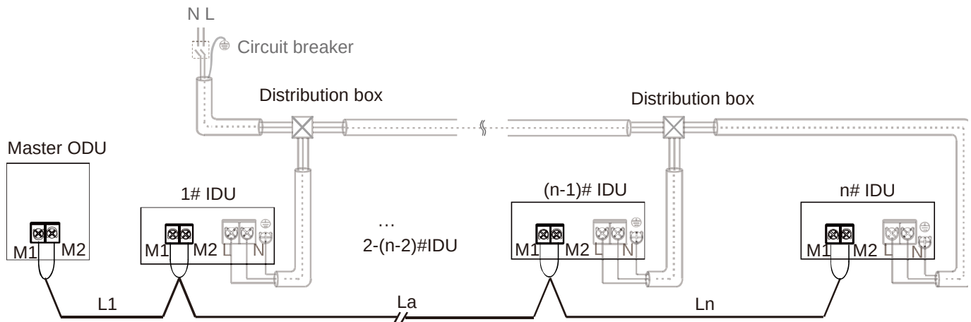
Figure 3-9.9: M1 M2 communication wiring configuration – IDUs uniform power supplied
