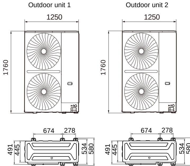
Figure 2-2.7: 34/36/40/42/44/46/48HP dimensions (unit: mm)
