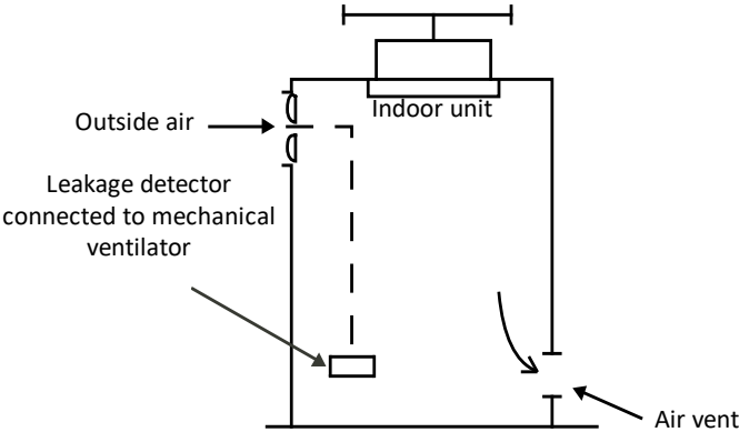
Figure 3-4.6: Mechanical ventilator controlled by refrigerant leak detector
