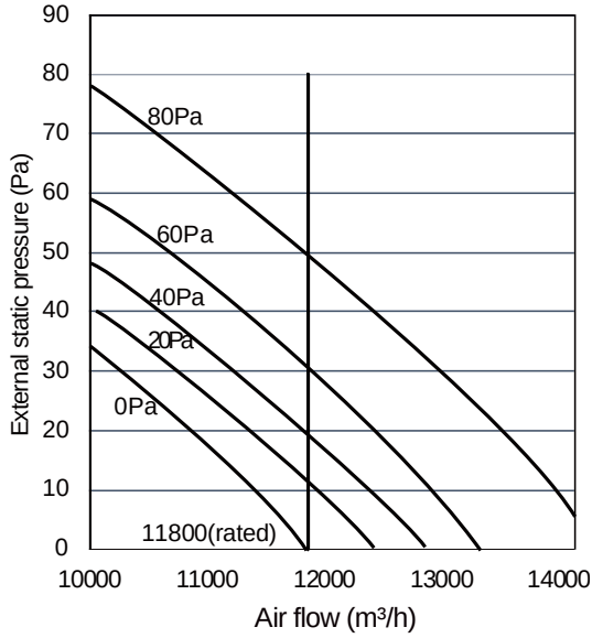
Figure 3-3.2: 8HP units fan performance
