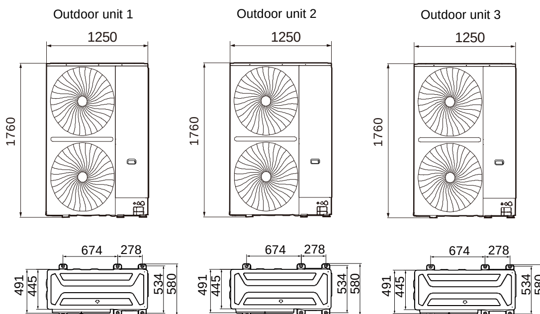
Figure 2-2.10: 54/58/60/62/64/66/68/70/72HP dimensions (unit: mm)
