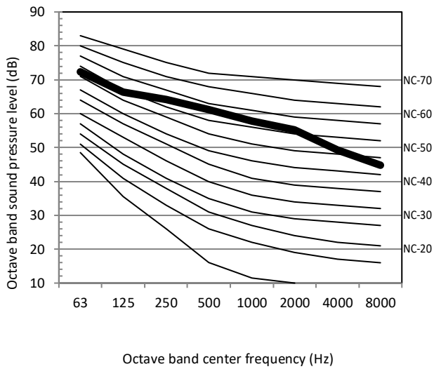
Figure 2-10.10: 24HP octave band level
