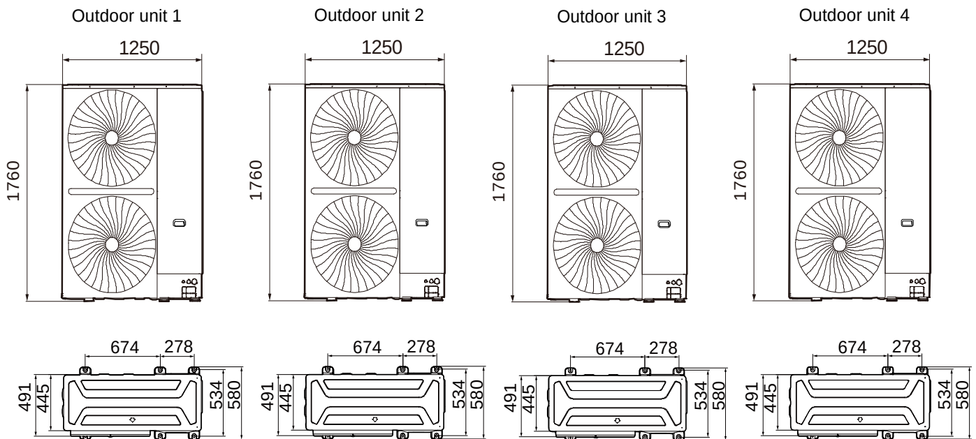
Figure 2-2.12: 76/78/80/82/84/86/88/90/92/94/96HP dimensions (unit: mm)
