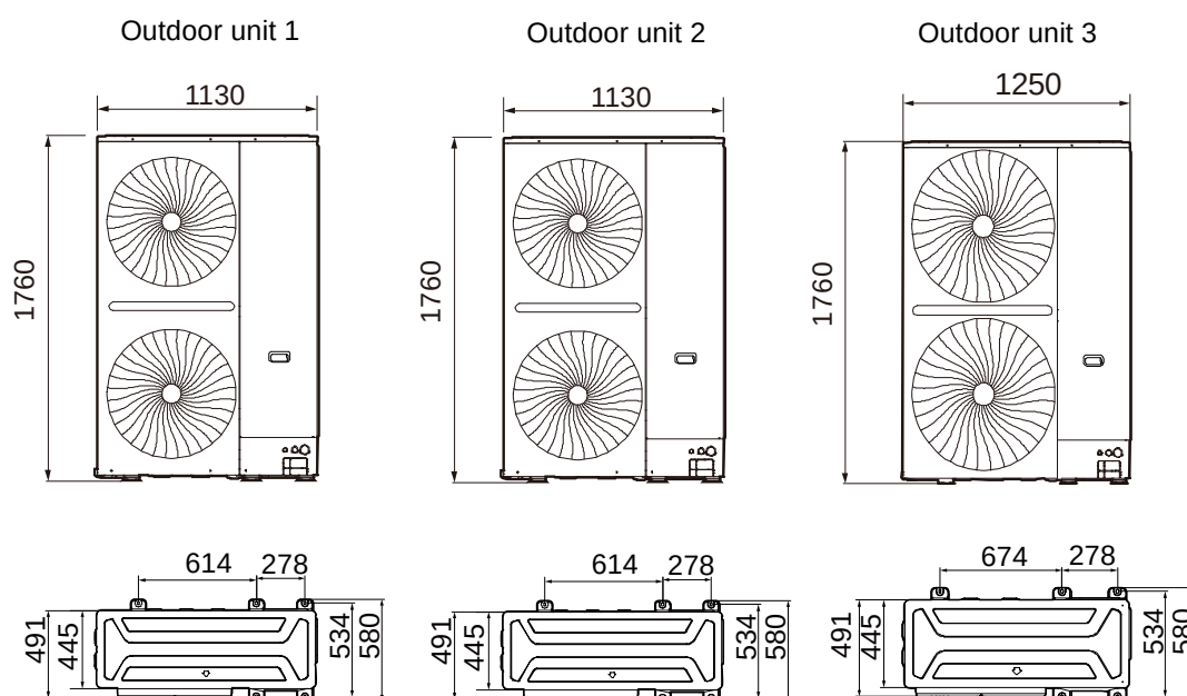
Figure 2-2.9: 52HP dimensions (unit: mm)
