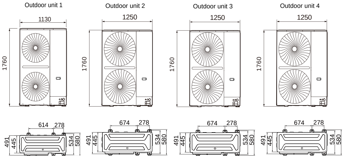
Figure 2-2.11: 74HP dimensions (unit: mm)
